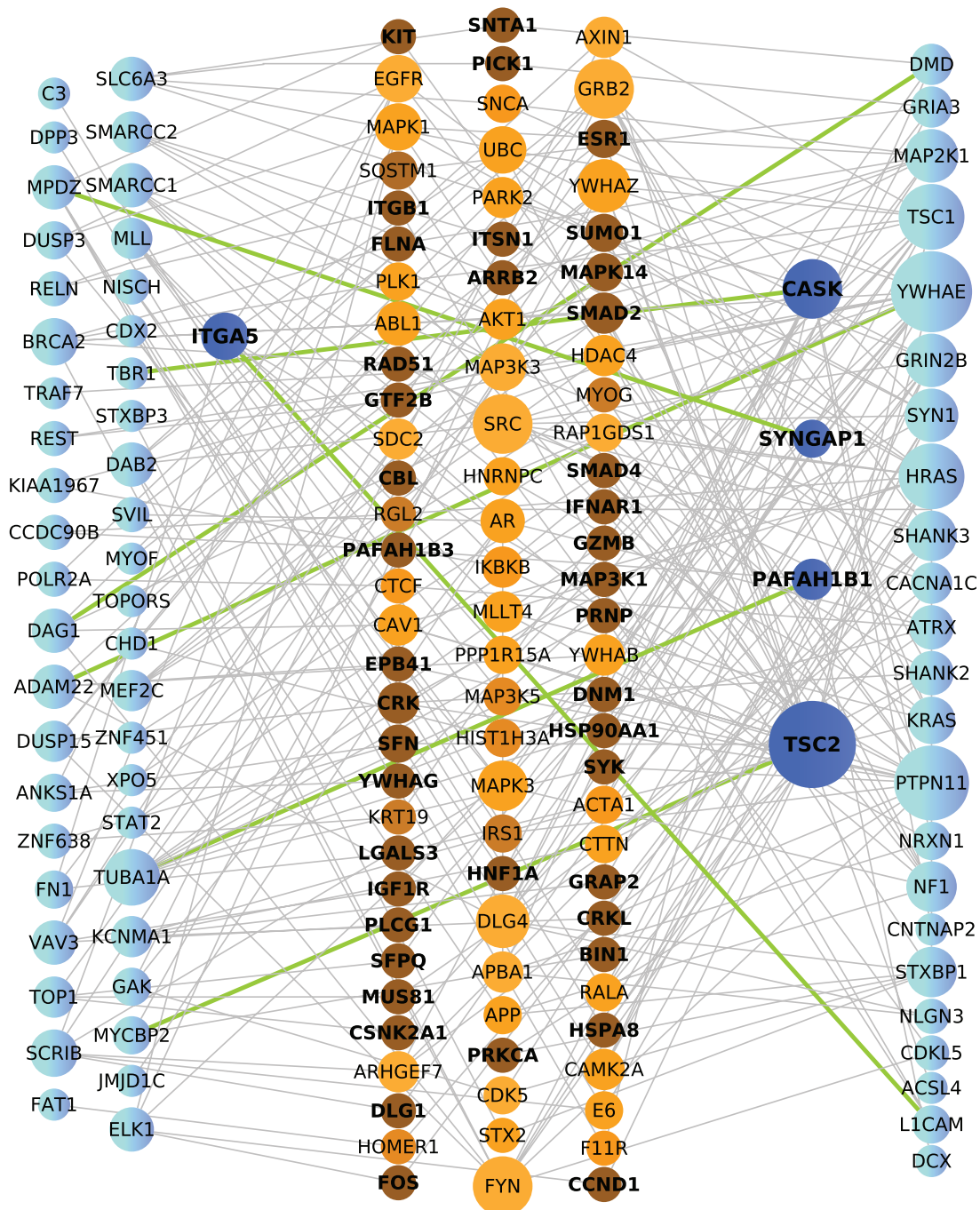
Figure 2. PPI network analysis for de novo variants and prior ASD genes (ASD112). Nodes are sized based on connectivity. Genes harboring de novo variants (left) and prior ASD genes (right) are colored blue with dark blue nodes represent genes that belong to one of these lists and are also intermediate proteins. Intermediate
